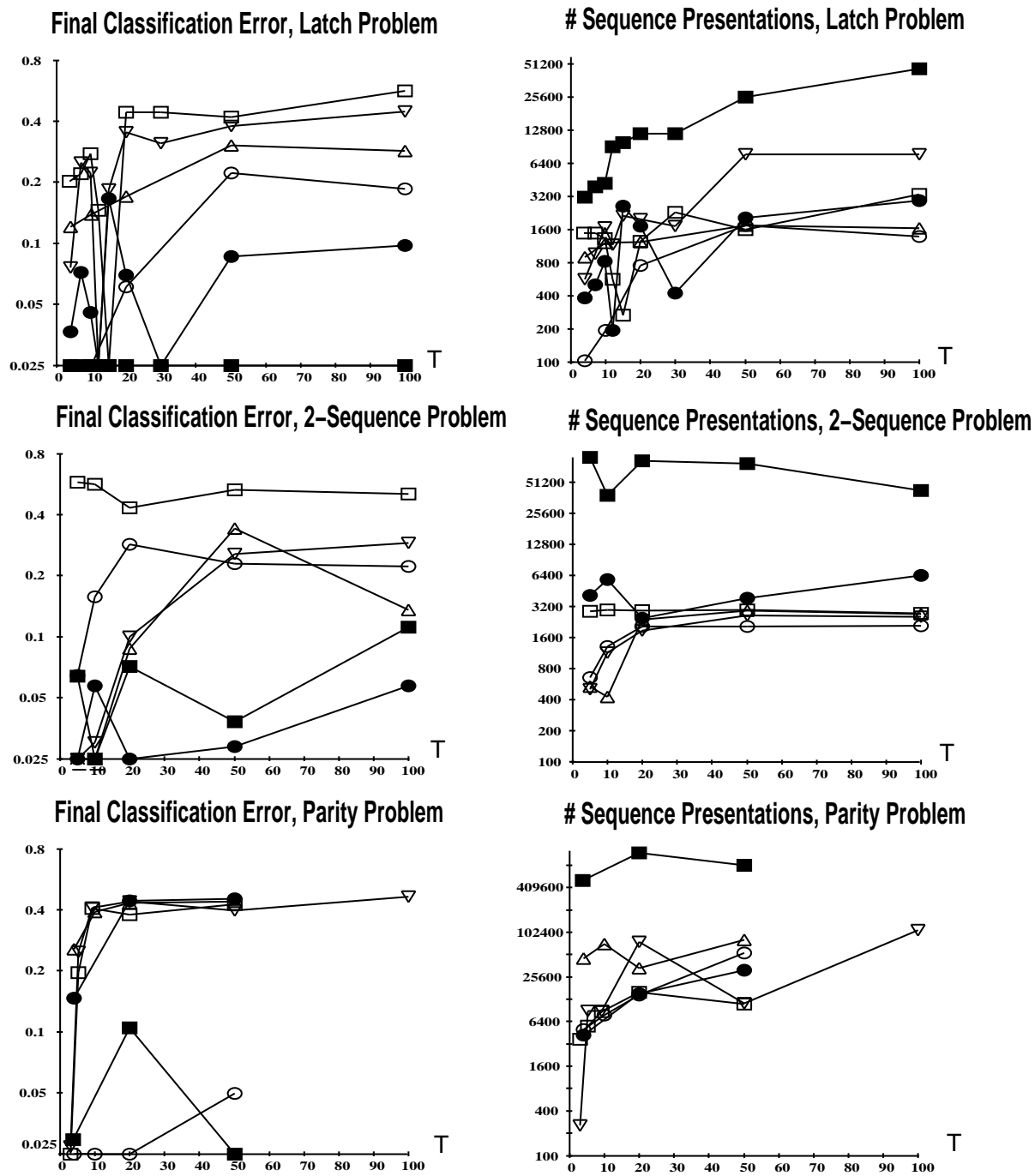
Figure 4: Comparative simulation results for: □ standard back-propagation, ▽ pseudo-Newton, △ time-weighted pseudo-Newton, ○ discrete error propagation, ● multi-grid random search, ■ simulated annealing. The horizontal axis ( T ) represents maximum sequence length. On the left, the vertical axis represents classification error after training; on the right, the number of sequence presentations to reach a stopping criterion.
